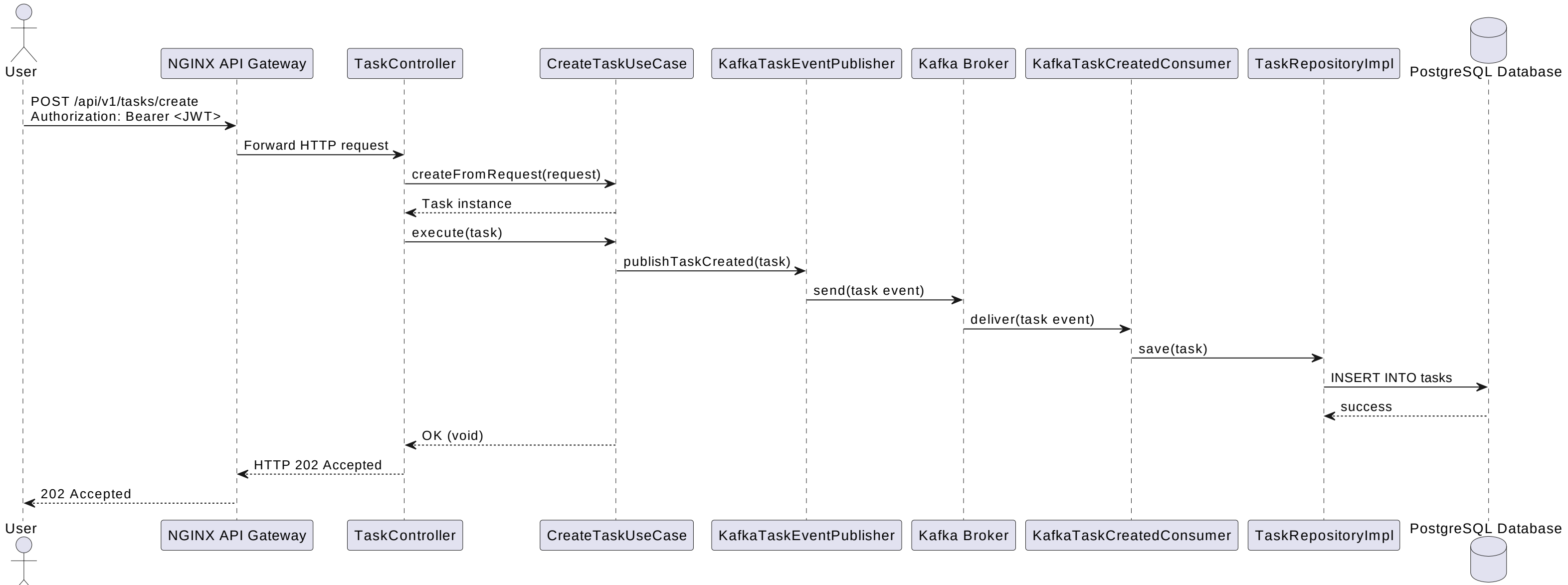
Sequence Diagram - POST /api/v1/tasks/create Clean Architecture Flow
